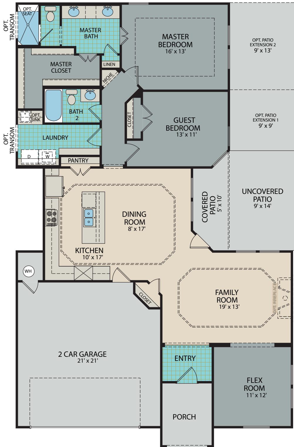
Floor Plan
