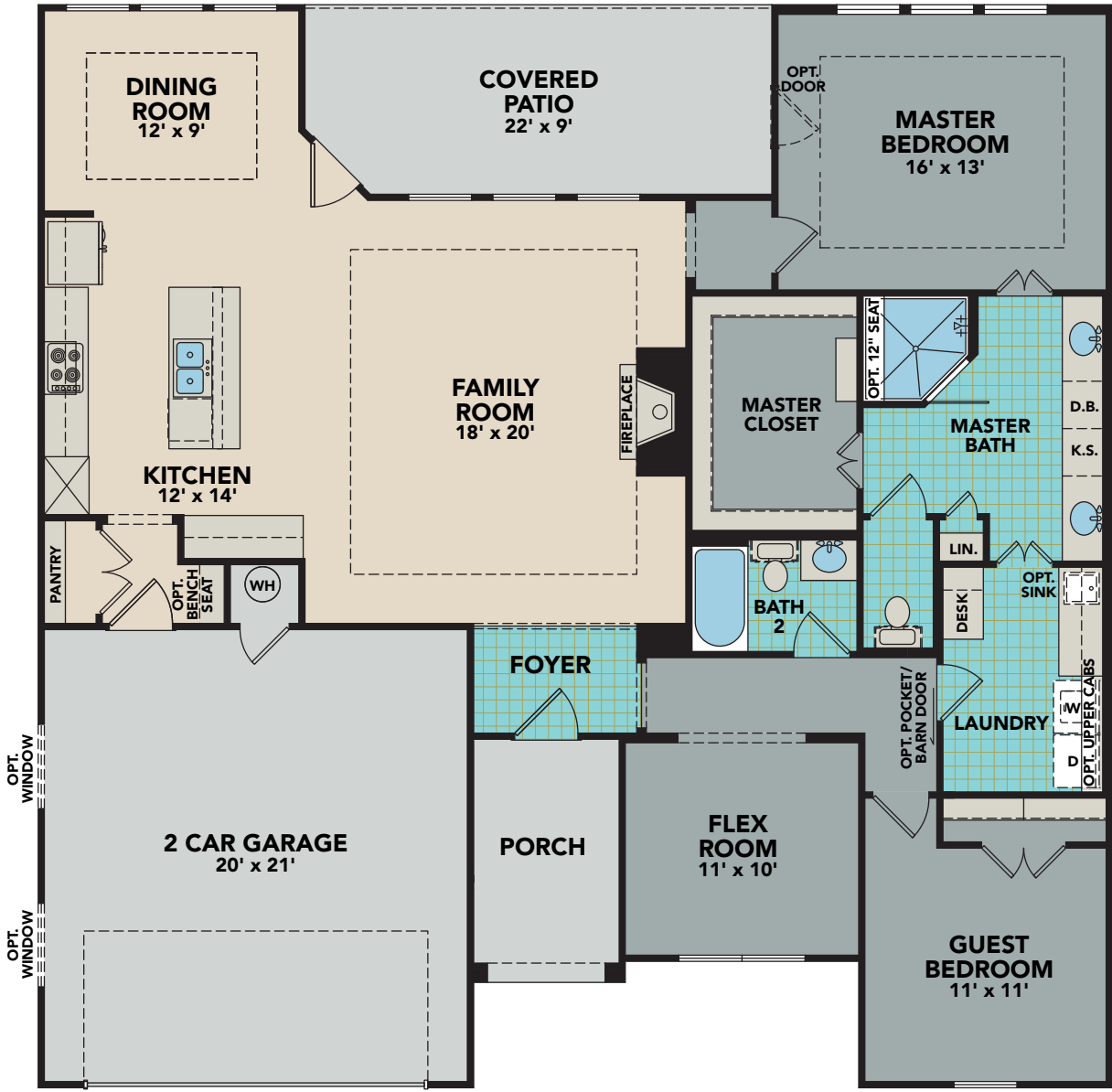
Floor Plan
